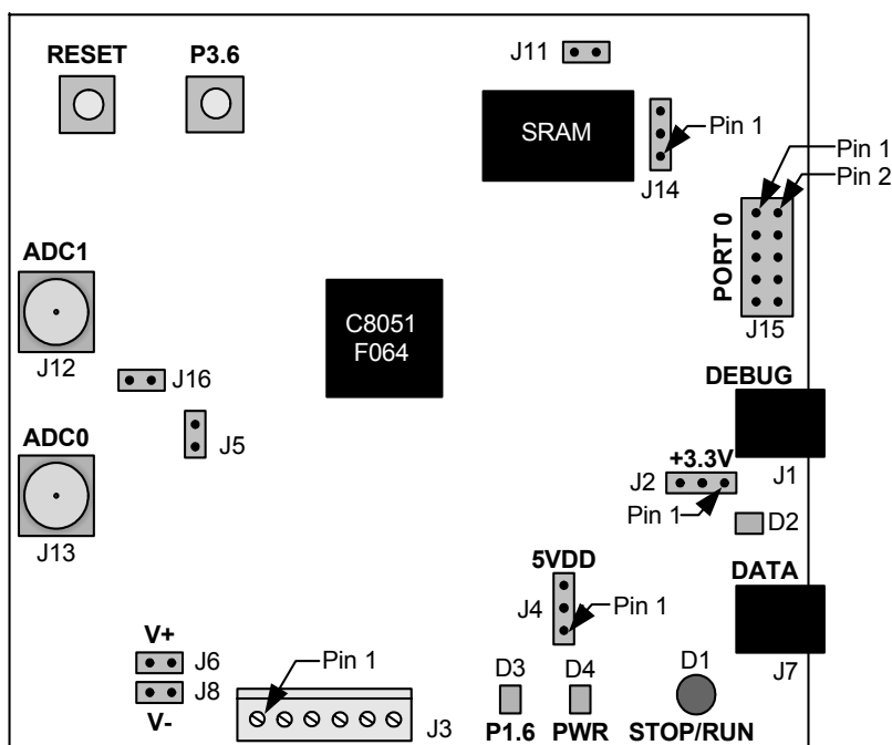
Figure 3. C8051F064 Evaluation Board
